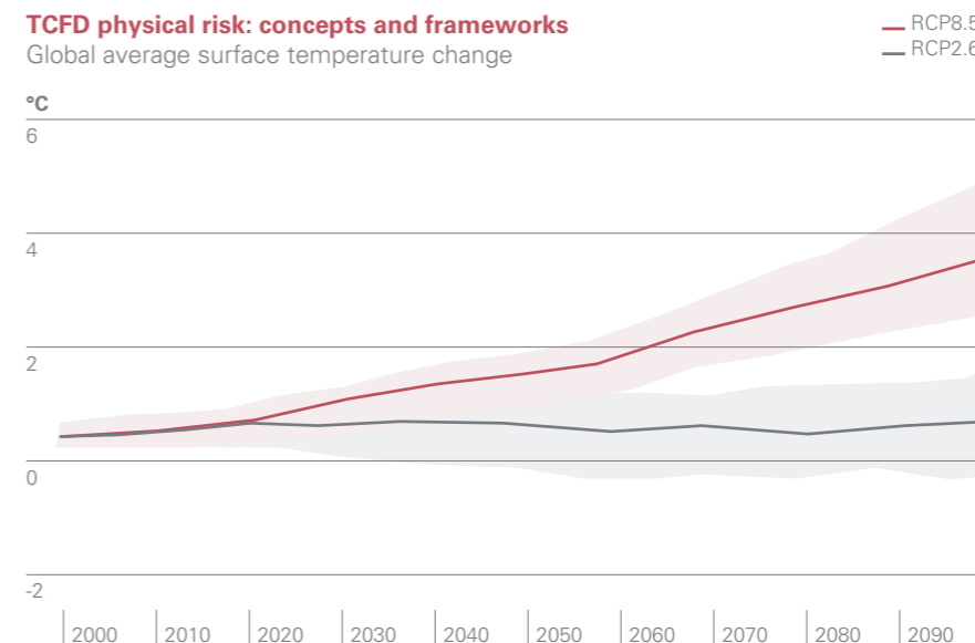
1. Climate model projections of average global temperature under the RCP2.6 and RCP8.5 scenarios (IPCC Fifth Assessment Report, 2013)
